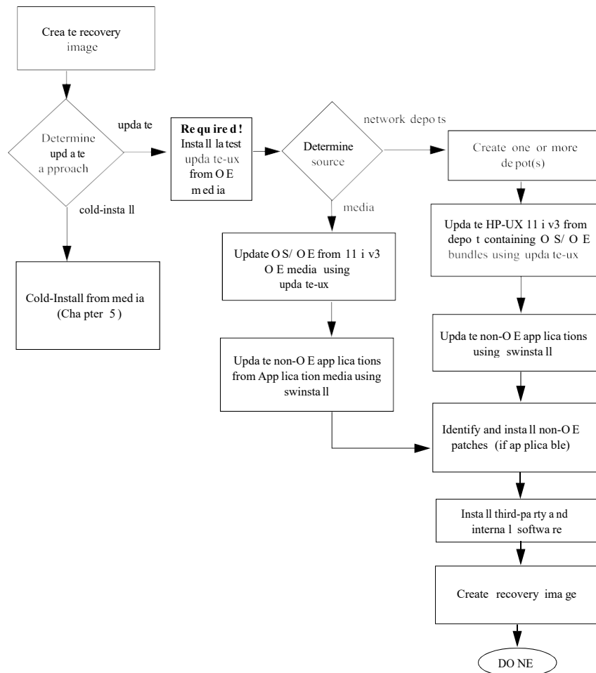
Figure 2: Updating to HP-UX 11i v3
