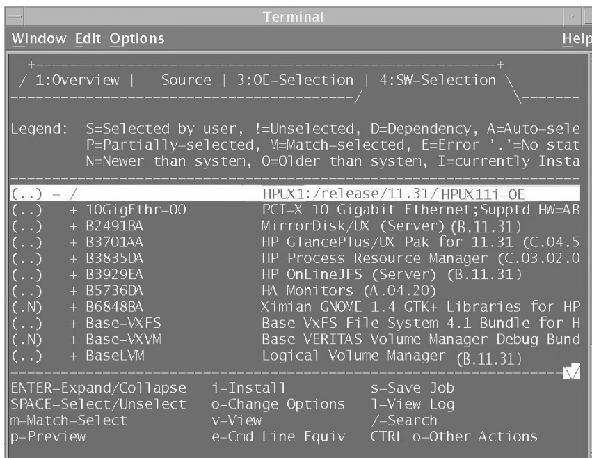
Figure 6: Software Selection Tab
