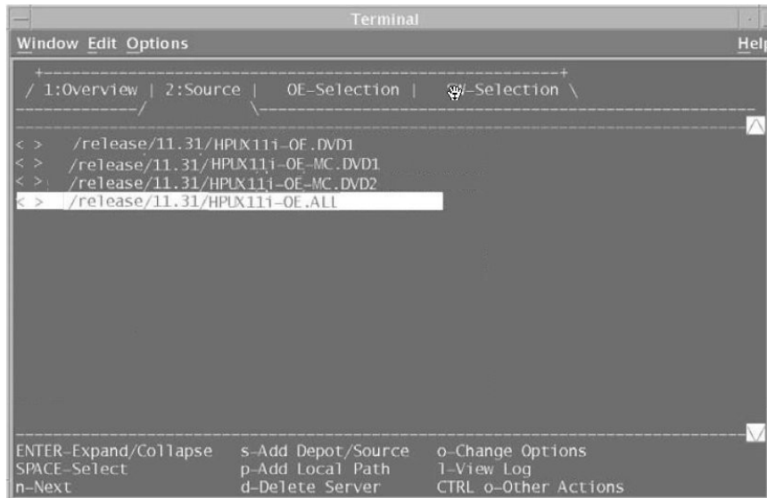
Figure 4: Select Source Tab
