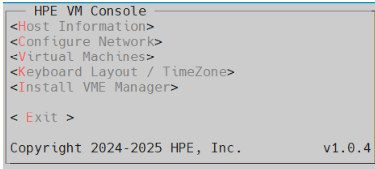
Figure 18. HPE-VM console
