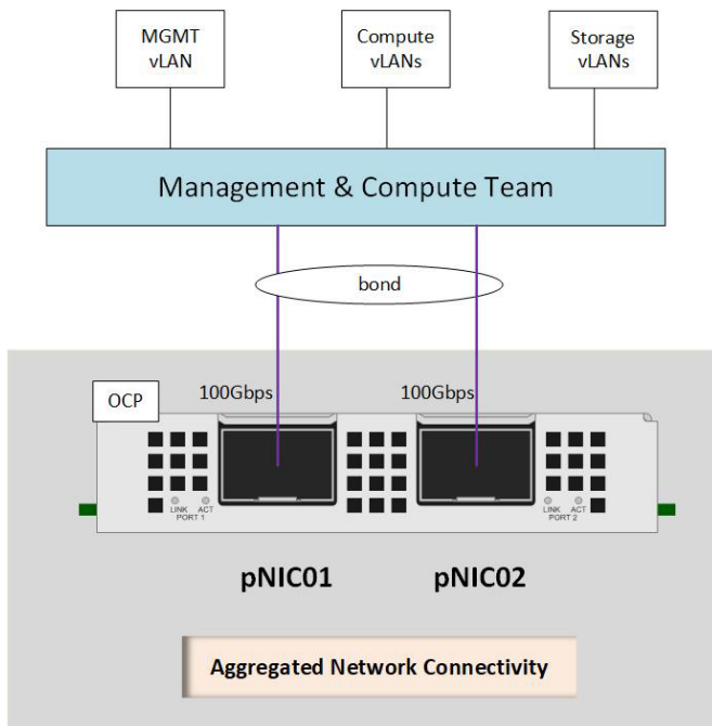
Figure 11. Aggregated Network Connectivity
