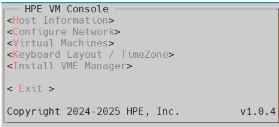
Figure 20. HPE-VM console
