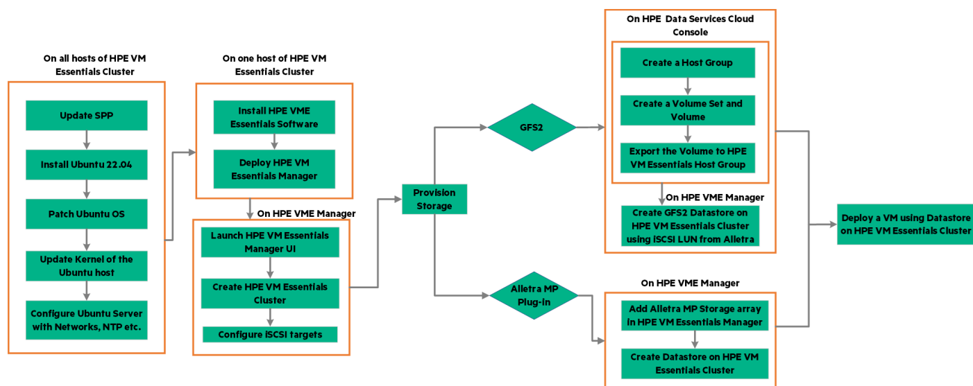
Figure 14. Workflow
