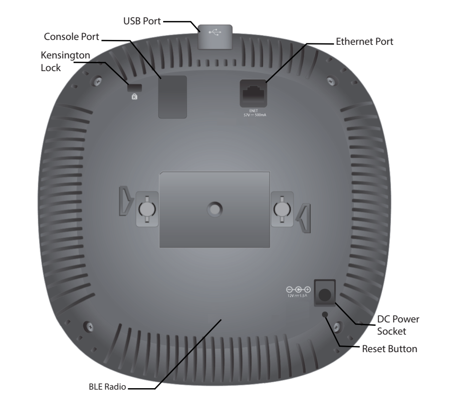
Figure 4 Back Panel
