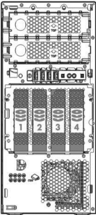
4-Bay LFF non-hot-plug drive model
