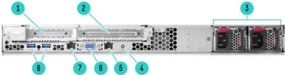
Rear View
