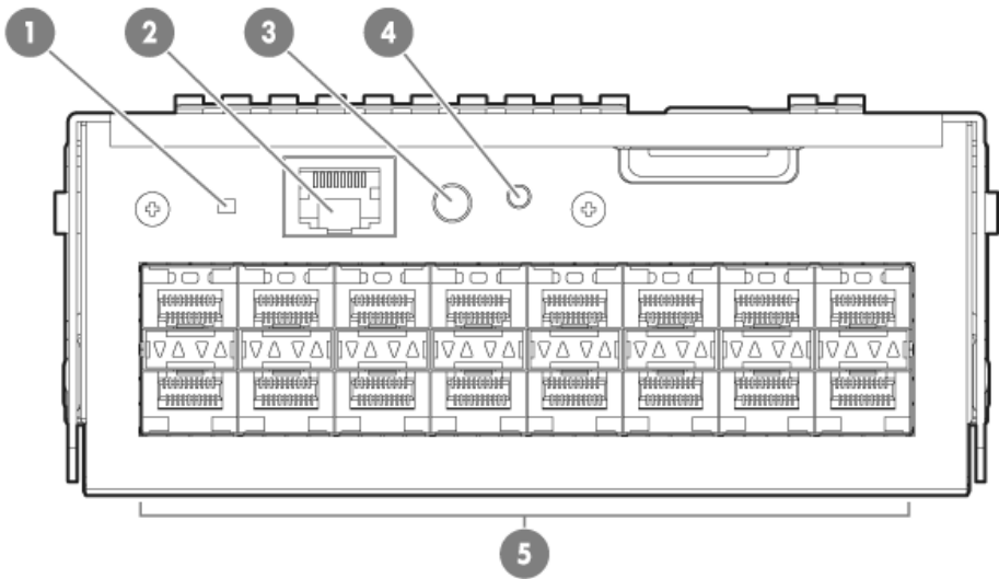
16SFP+ Uplink Module Components
