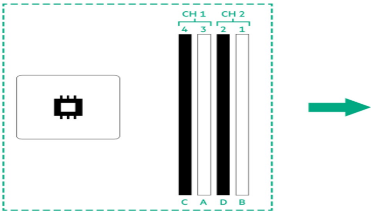
UDIMM maximum configuration (1 CPU model)
