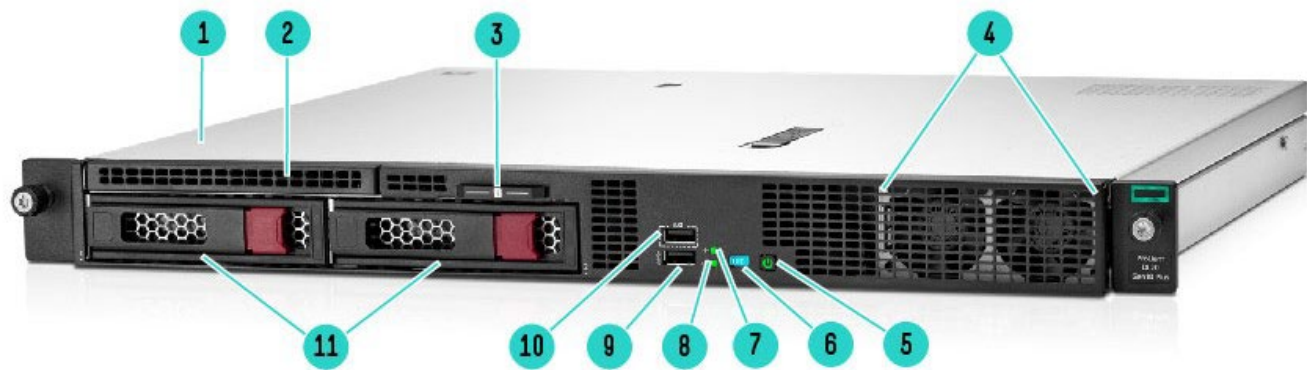
2 LFF Front View Gen10 Plus
