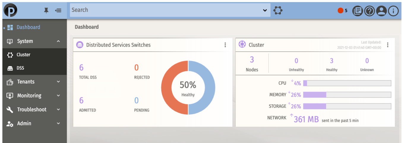
Figure 4. AMD Pensando PSM interface, showing the dashboard, with the “System” section of the main menu open; its two subsections, “Cluster” and “DSS”, are visible and selectable.
