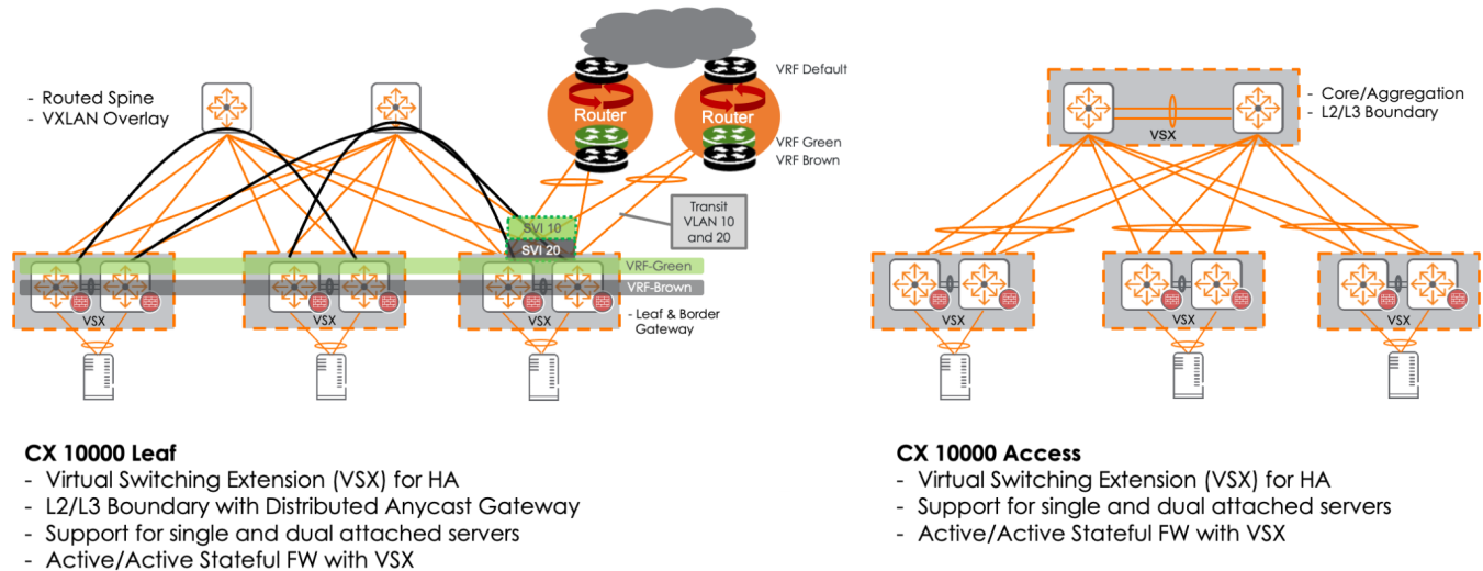
Figure 36. Deployment architectures
