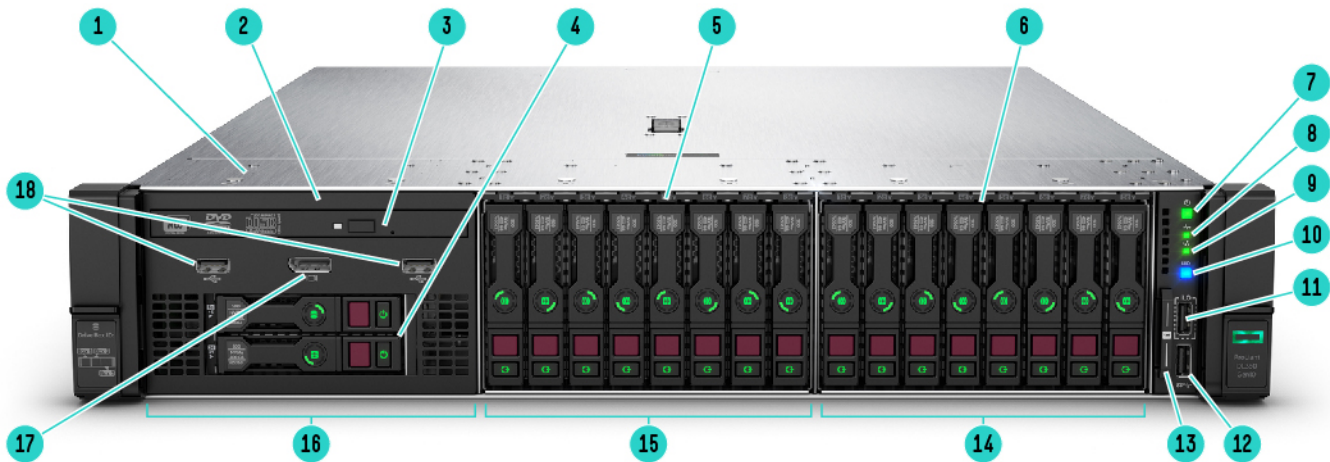
HPE ProLiant DL385 Gen10 Server - Front View SFF chassis with optional Universal Media bay with optical and 2 NVMe plus 16 NVMe shown
